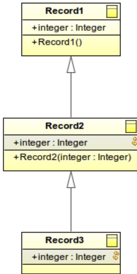
Figure 3.2 Record3 cannot be instantiated with the default constructor because Record2 declares a constructor so it is not possible to use its default constructor and it does not declare a non-parametric constructor
