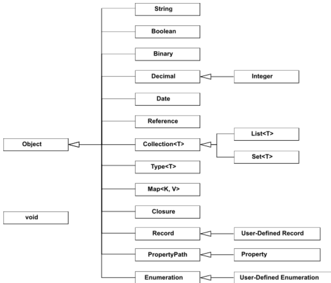
Figure 3.1 Type hierarchy of built-in types
