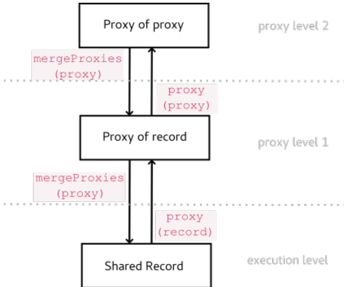
Figure 2.84 Proxy levels: Proxy object of the shared record exists on proxy level 1. It can see the record and any other data in its context. The proxy of the proxy lives on proxy level 2: It can see proxy level 1 and the original record; the proxy of record cannot see proxy level 2.
