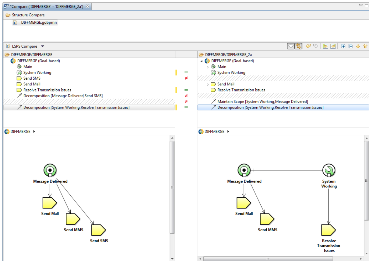
Figure 2.40 Comparing goal-based Processes
