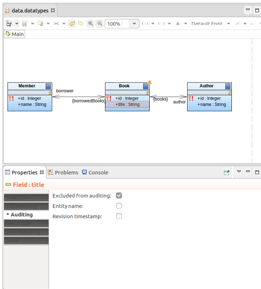
Figure 2.83 Field excluded from auditing
