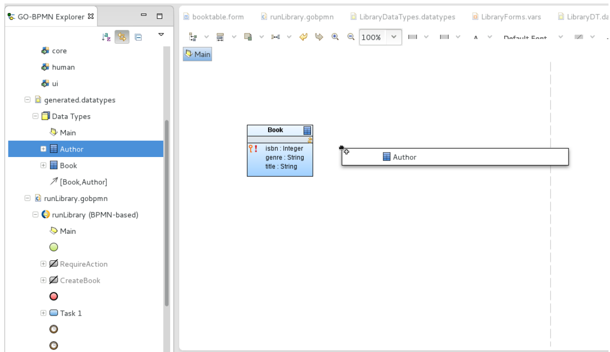
Figure 2.75 Adding a depiction of a generated shared record onto a data type diagram
