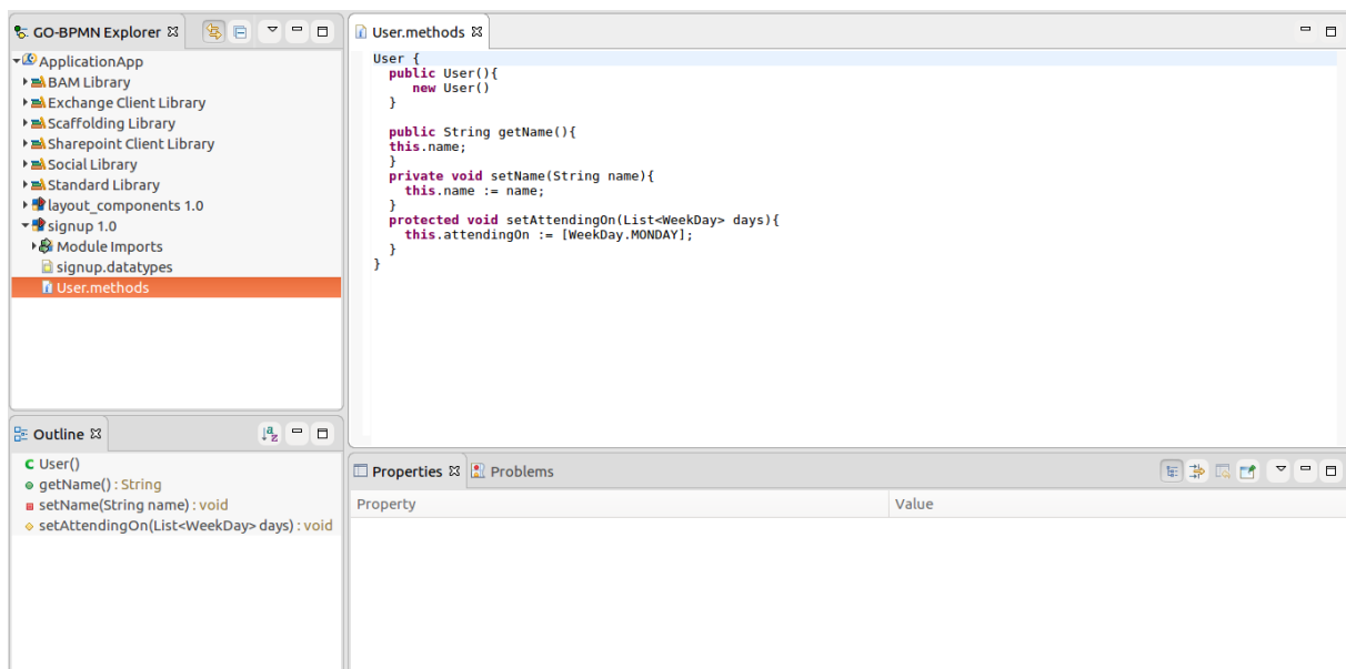
Figure 2.63 Method definitions: constructor and methods with different visibility
