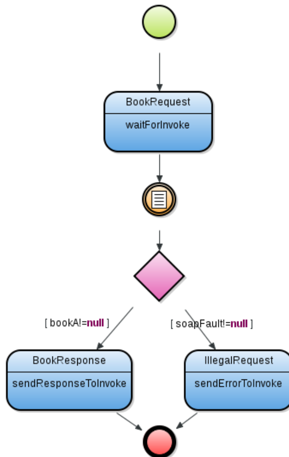
Figure 2.86 Workflow of a process serving as a web service server
