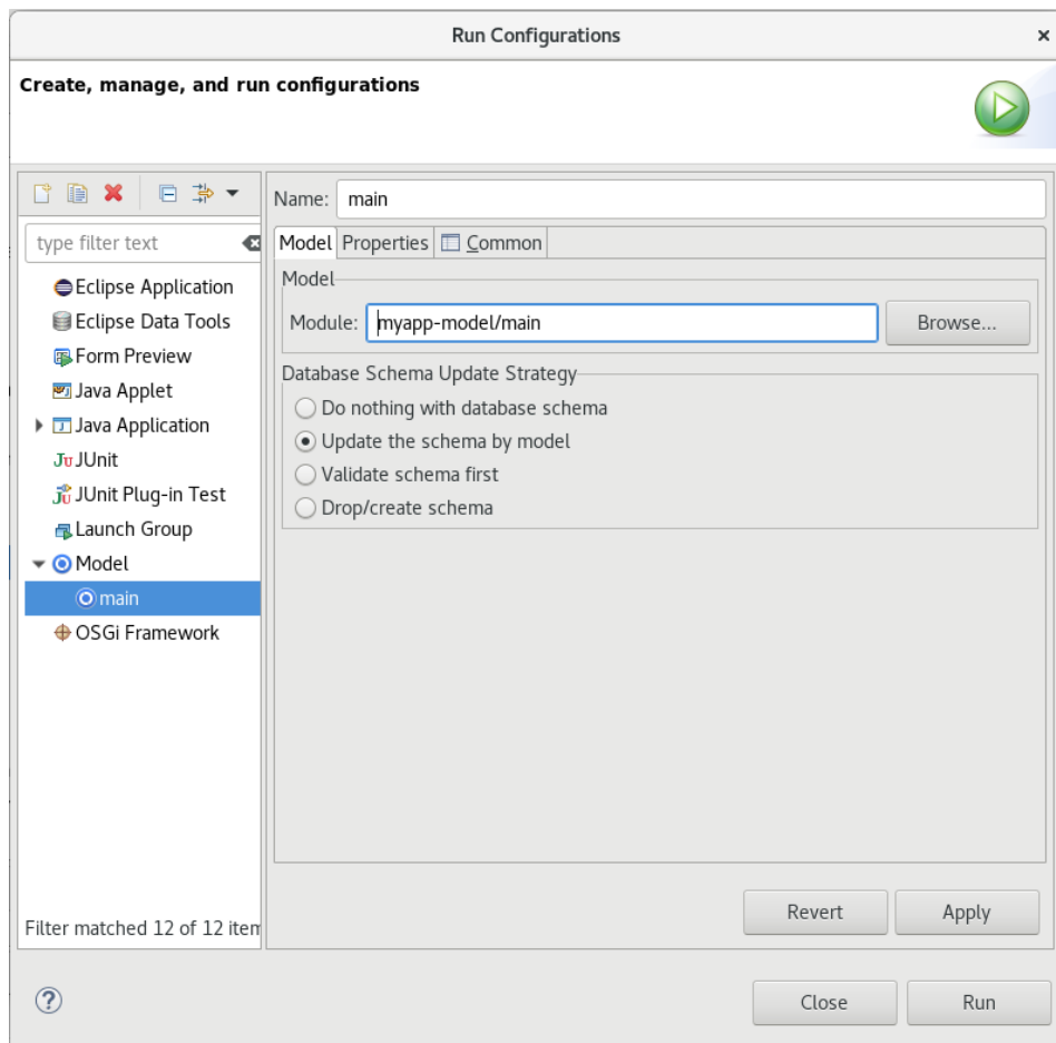
Figure 3.5 Run and upload configuration for the main module
