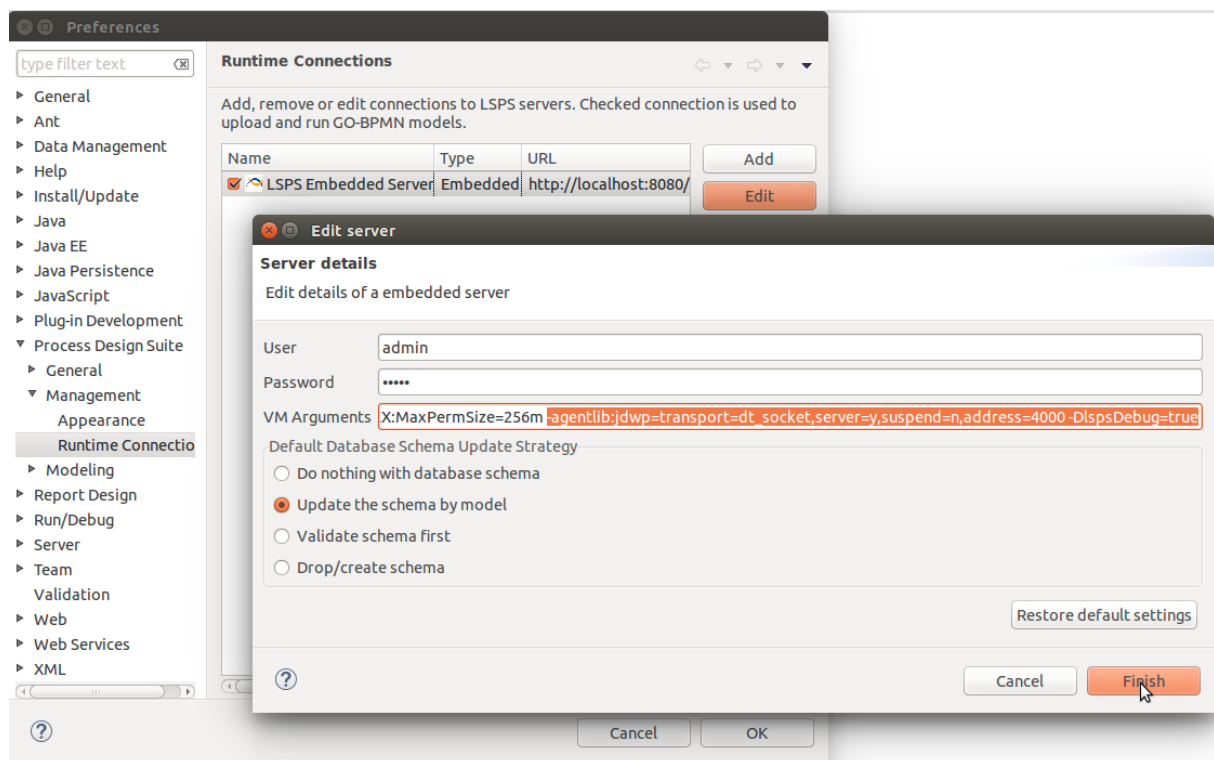
Figure 3.13 Debug parameters in PDS Embedded Server configuration
