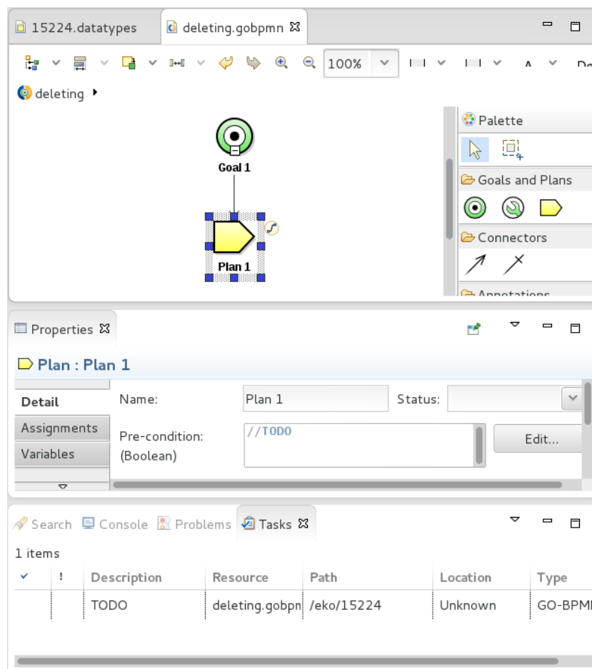
Figure 2.46 The TODO Marker
