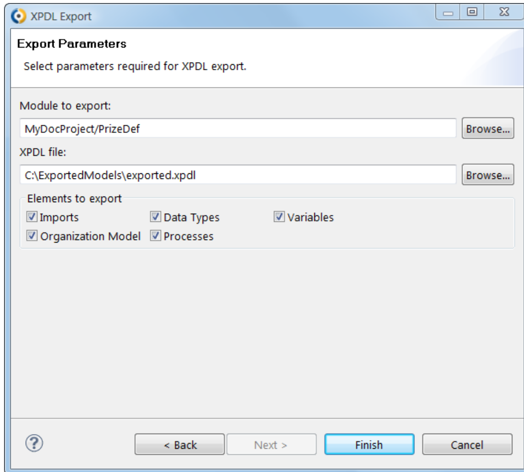
Figure 2.98 Defining XPDL Export settings
