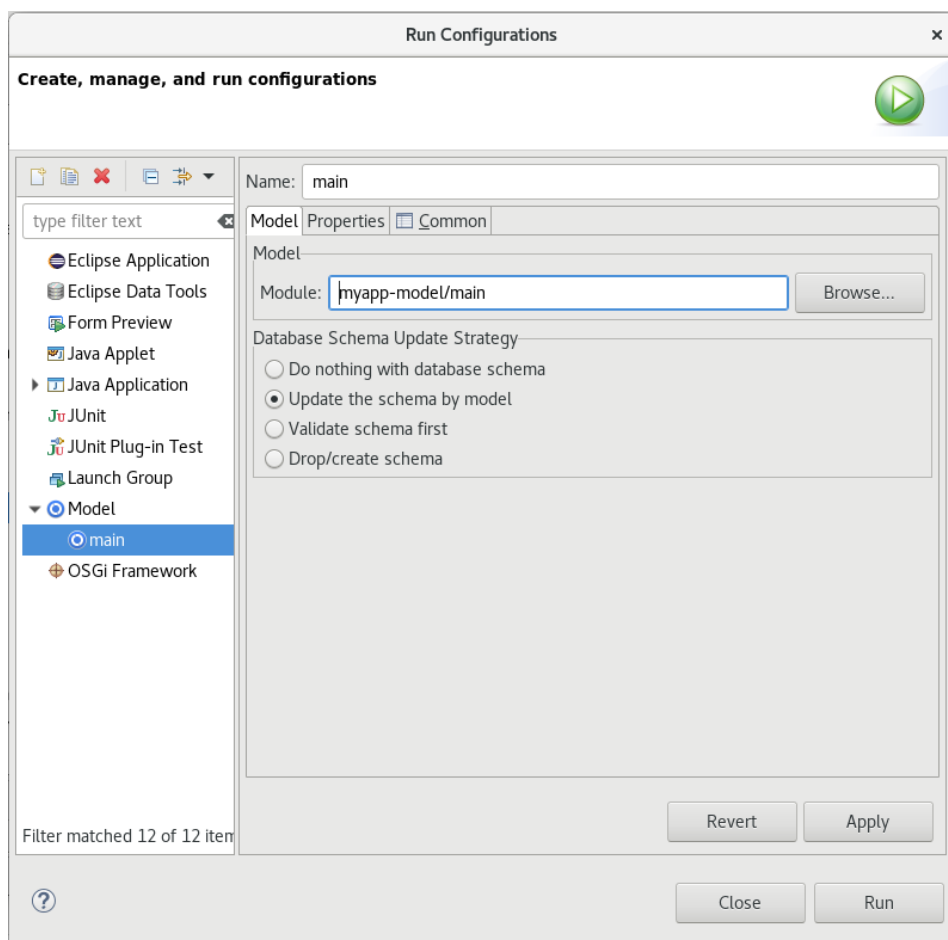
Figure 3.10 Run and upload configuration for the main module
