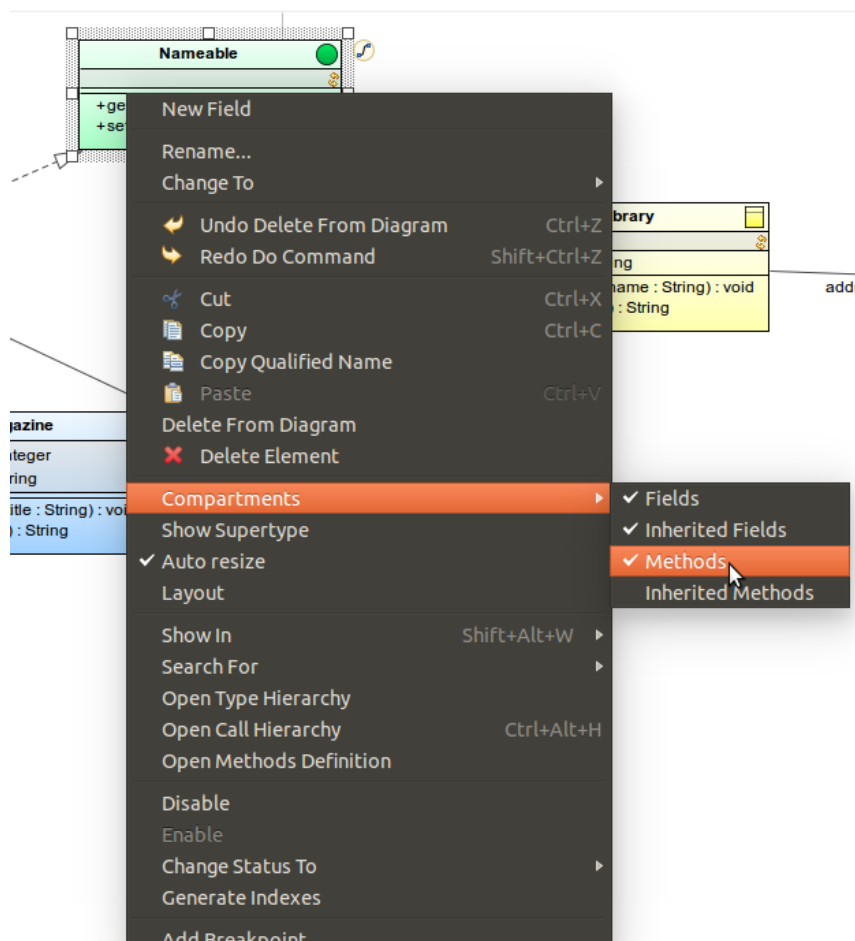
Figure 2.69 Available Record compartments
