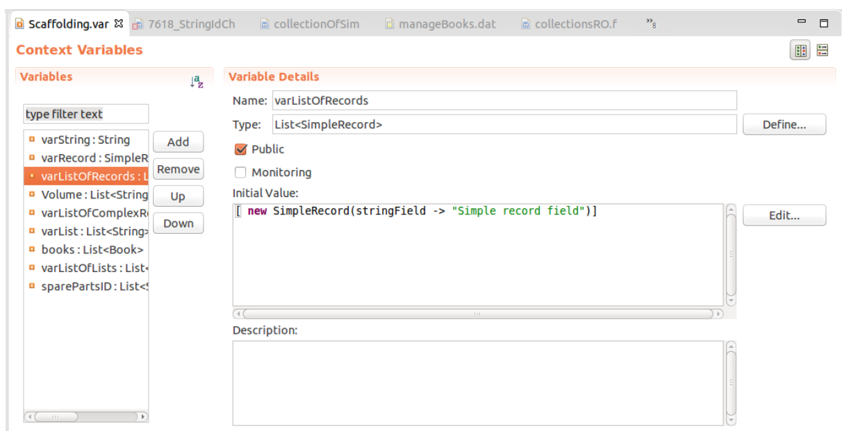
Figure 2.54 Editing variable definitions
