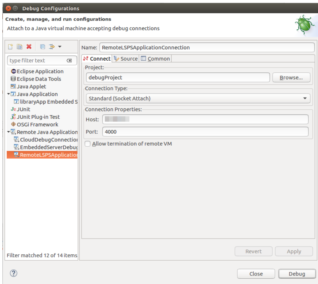
Figure 3.14 Setting debug configuration
