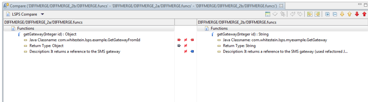
Figure 2.43 Comparing three resources
