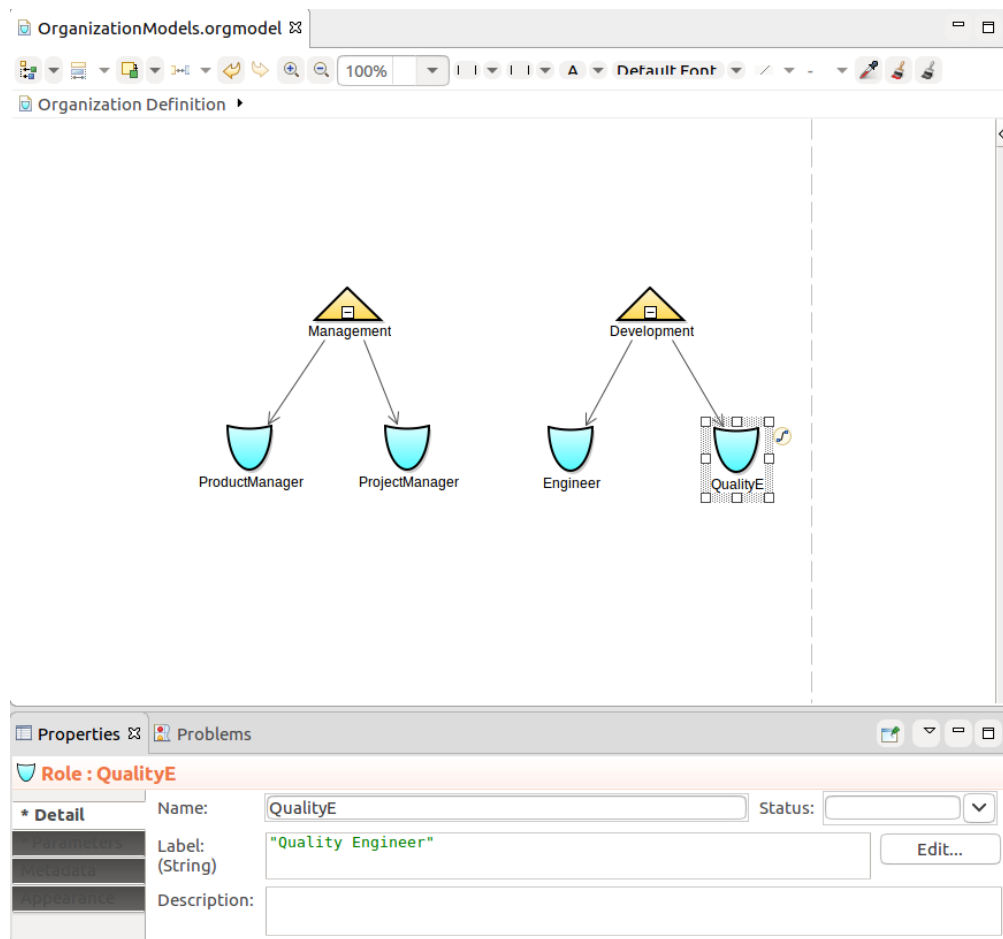
Figure 2.55 Editing the Main diagram of an organization definition file
