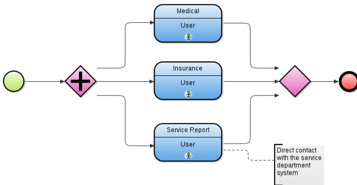
Figure 2.29 Diagram with tree line style
