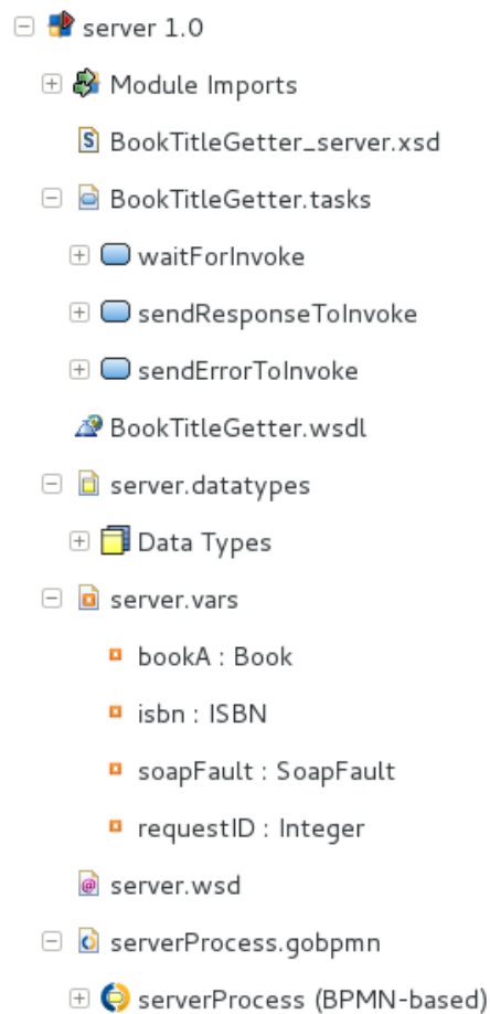
Figure 2.87 Web Server Service Module
