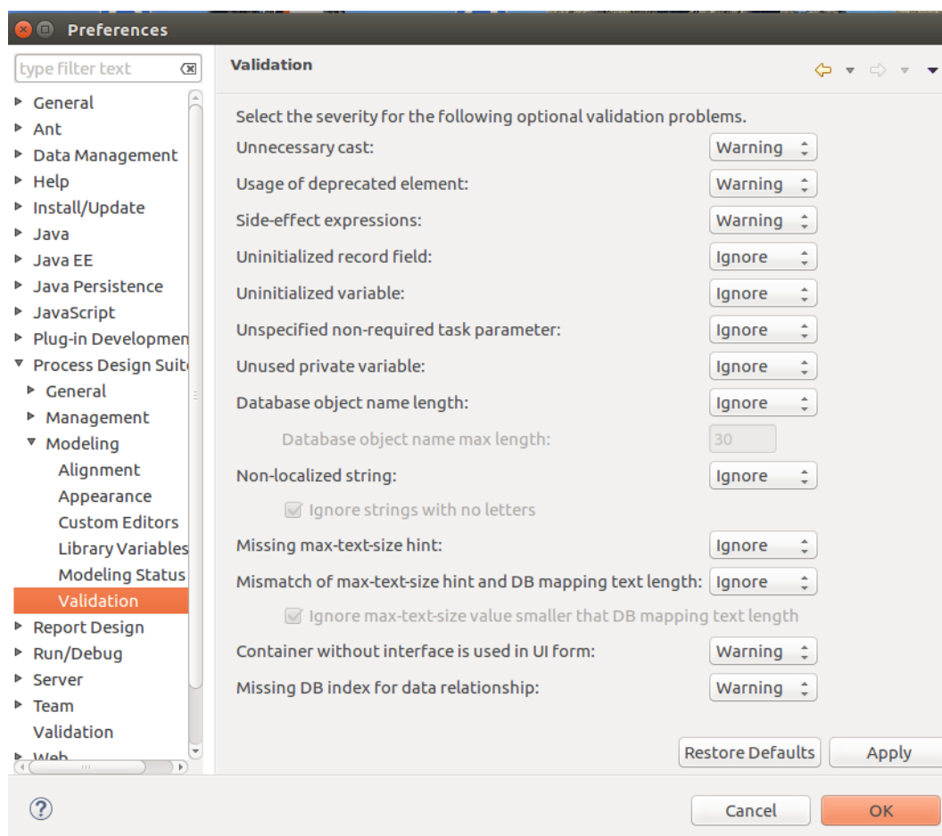
Figure 2.49 Validation page with predefined settings
