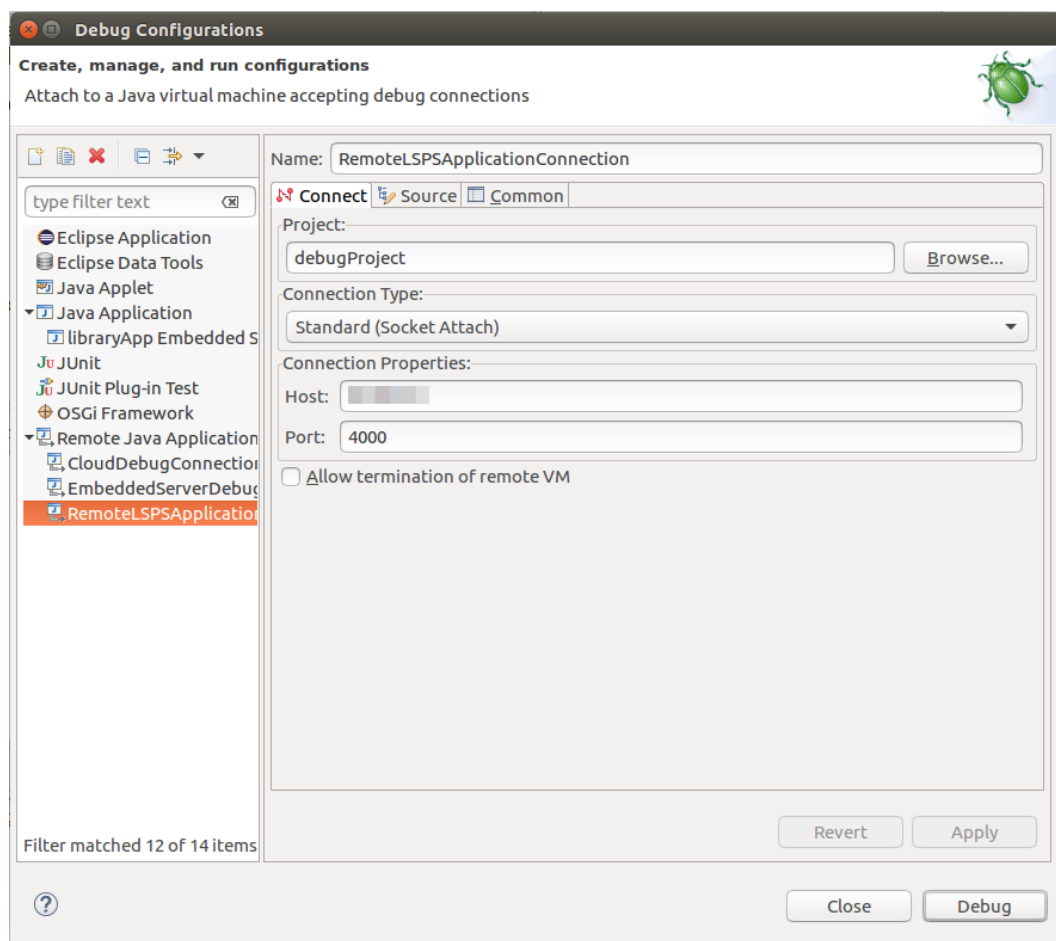
Figure 3.18 Setting connection to a remote server
