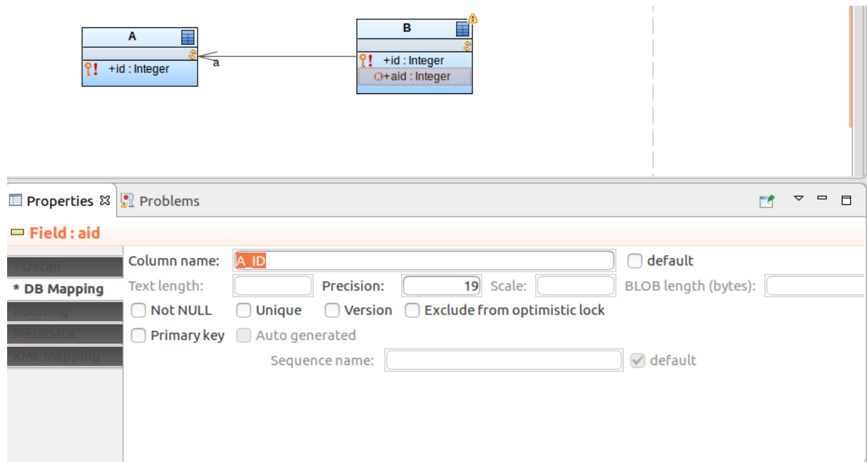
Figure 2.79 DB mapping of the field
