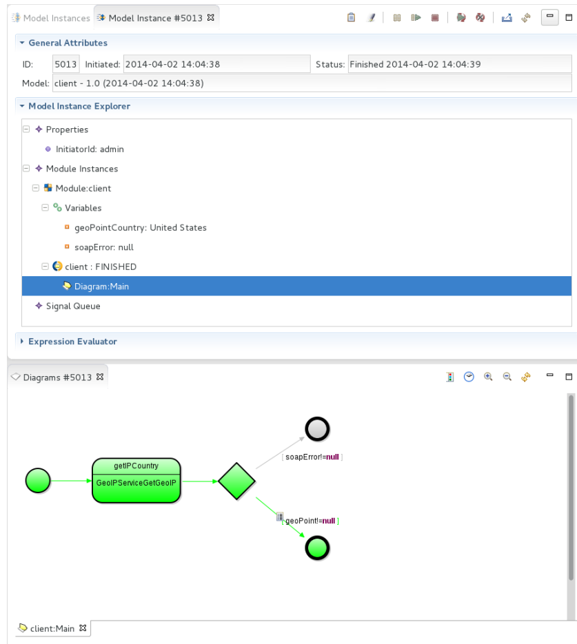
Figure 2.92 Model instance of a web service client Process
