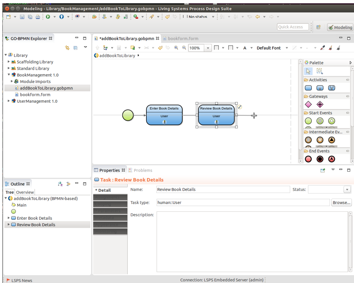
Figure 2.51 Creating Process workflow
