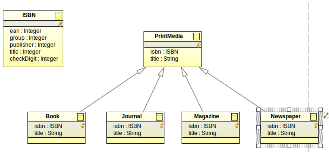
Figure 2.64 Hierarchy of Records with multiple subtypes
