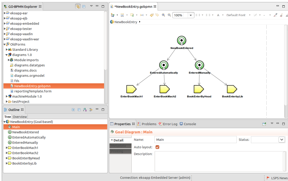
Figure 2.39 Goal diagram opened after Auto-layout was selected
