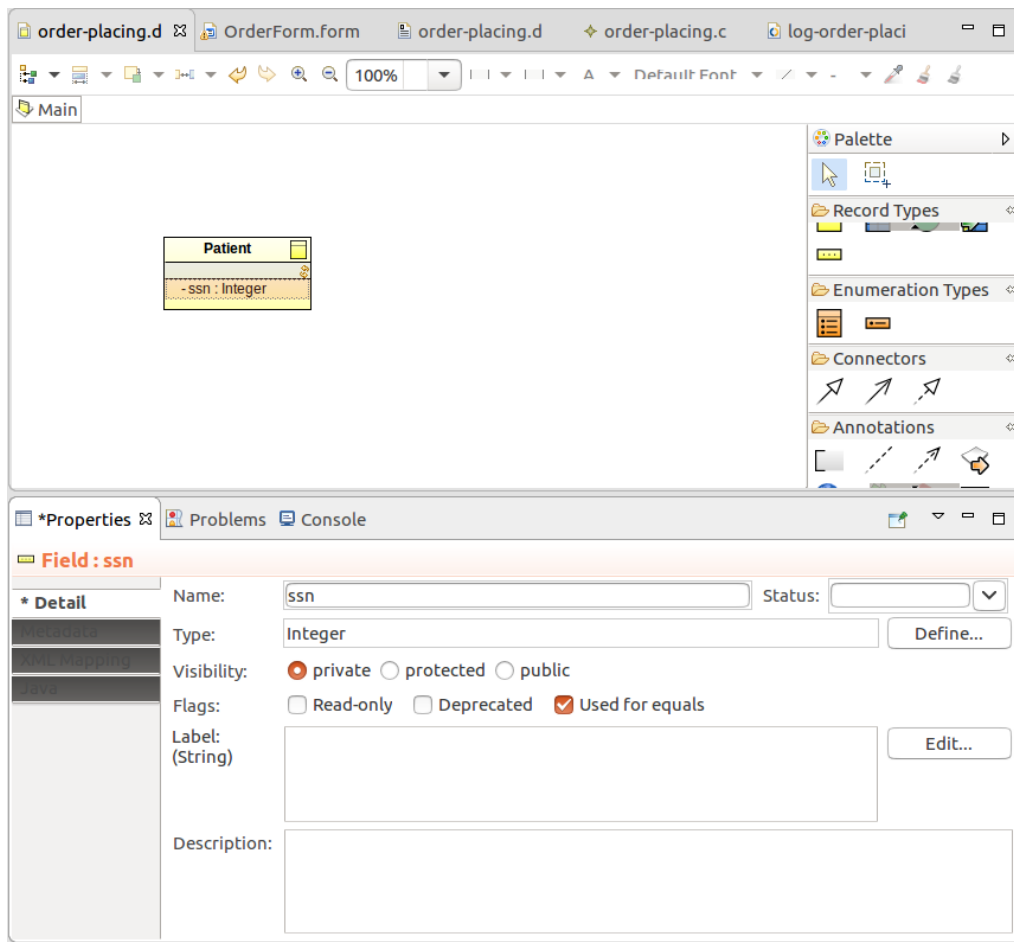
Figure 2.62 Field with its properties
