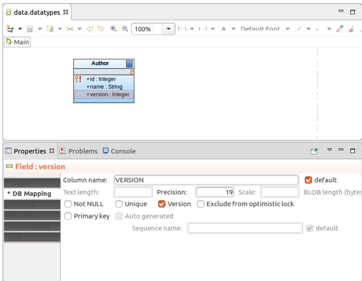
Figure 2.76 The Version field of a Shared Record
