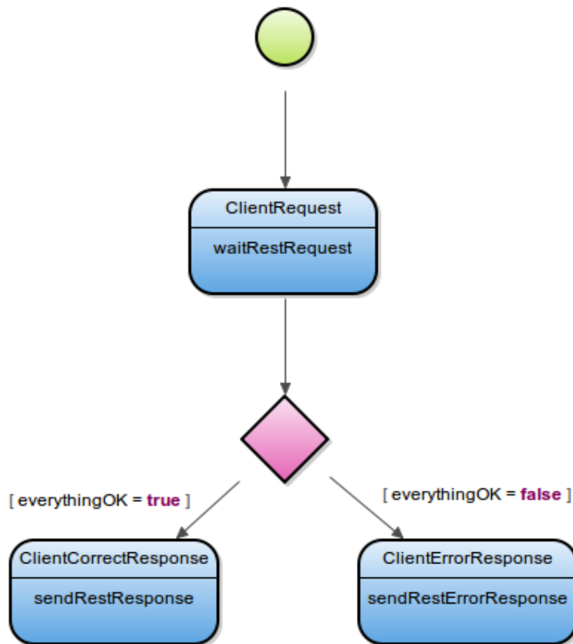
Figure 2.85 REST Server Process
