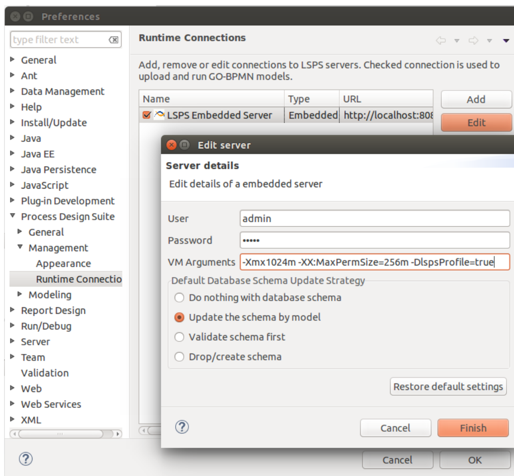
Figure 3.23 Profiler-enabling property on the Embedded Server connection setting
