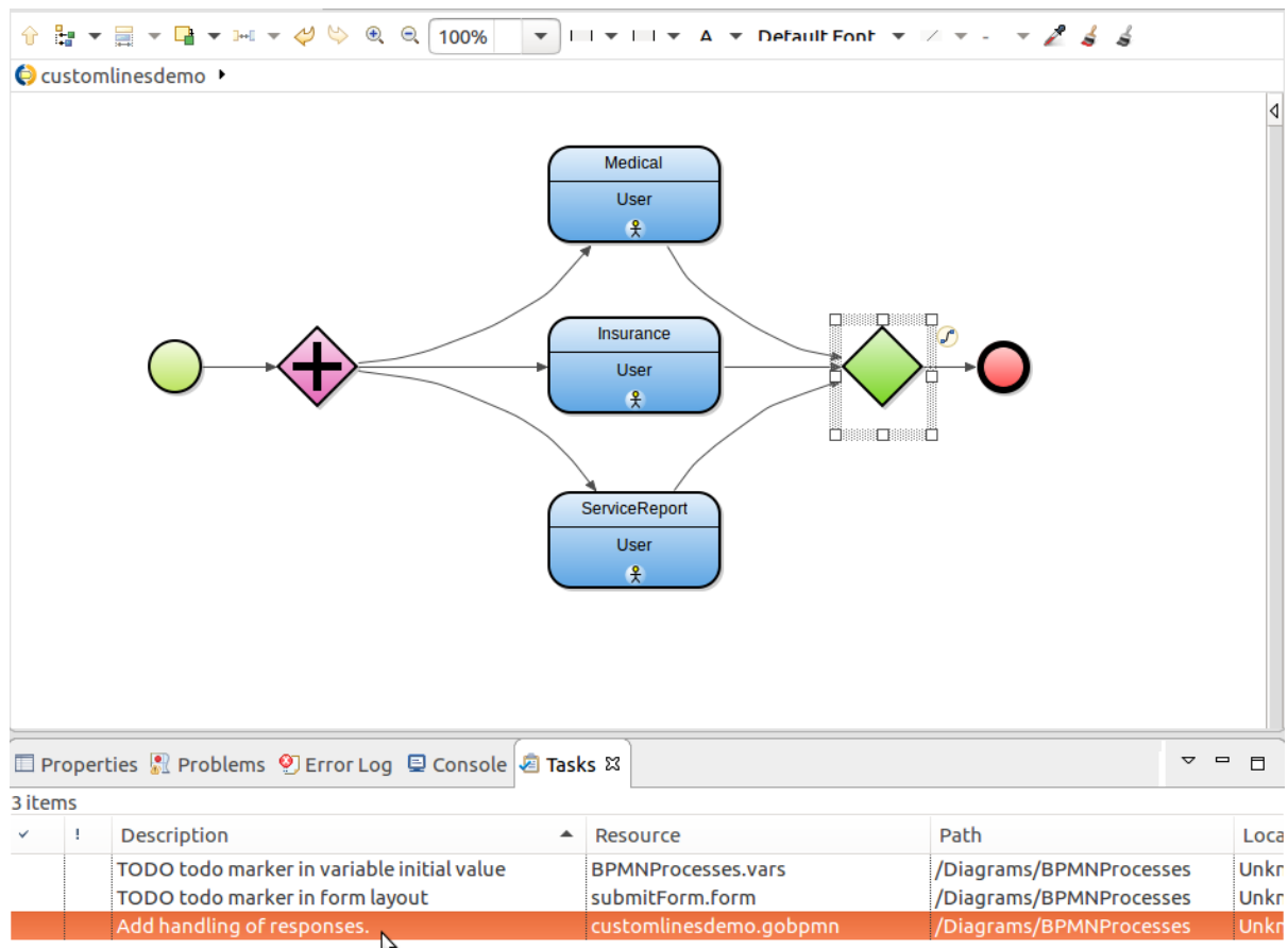
Figure 2.47 Modeling status with the normal priority on an element with its entry in the Tasks view
