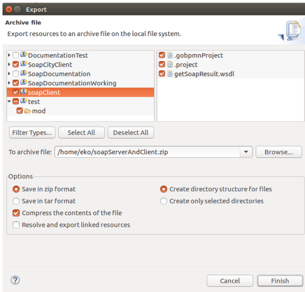
Figure 2.94 Selecting resources and files to be exported into an archive
