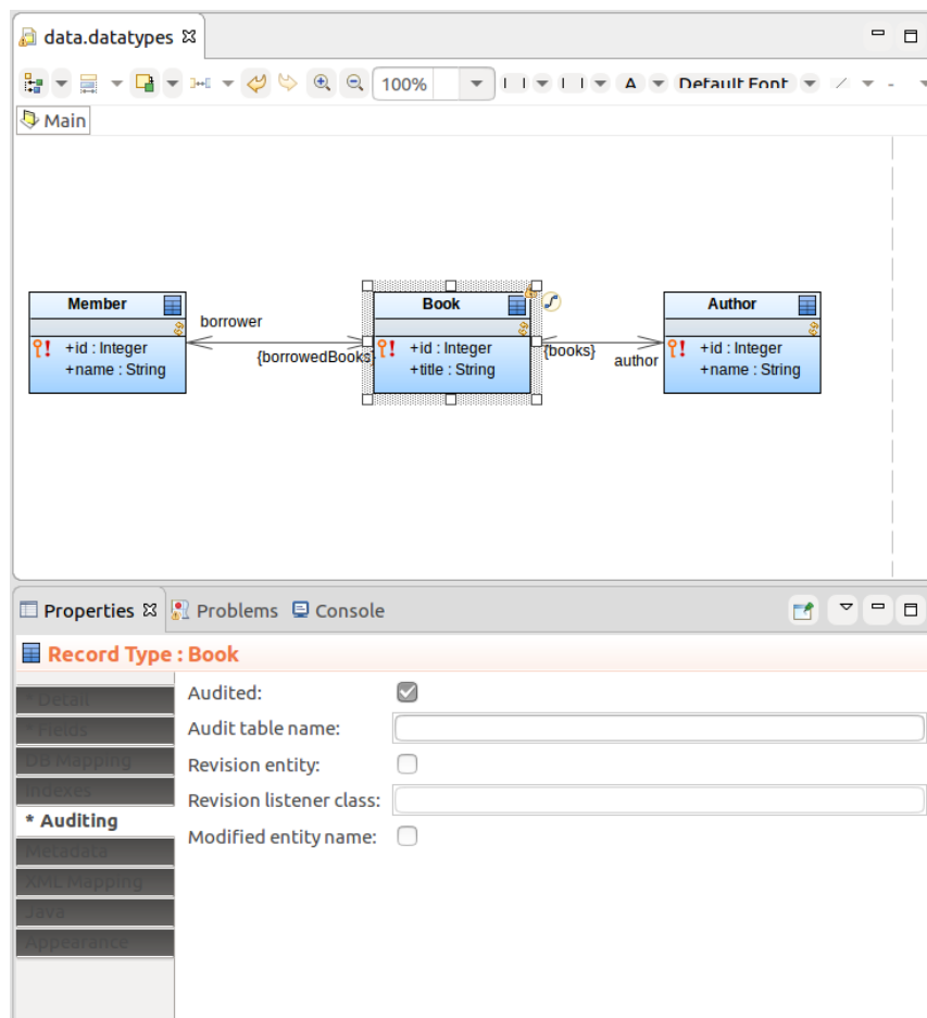
Figure 2.82 Audited shared Record
