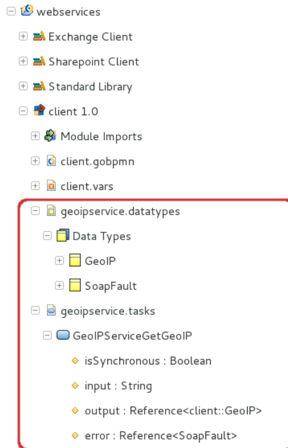
Figure 2.91 Generated Task Types and Data Types
