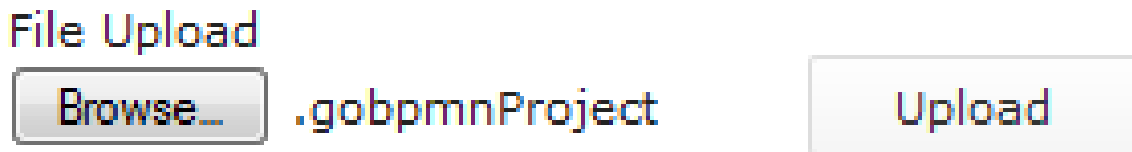
Figure 4.13 File Upload
